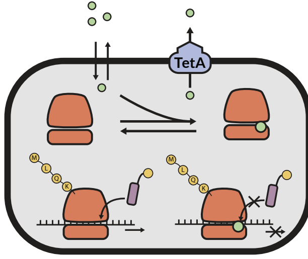
Figure 1: Mode of action for tetracycline and the efflux pump TetA. Tetracycline enters the cell passively and binds the small subunit of the ribosome, where it inhibits translation by blocking binding from the charged tRNA. TetA reduces the intracellular concentration of tetracycline by pumping out the drug against a proton gradient.
