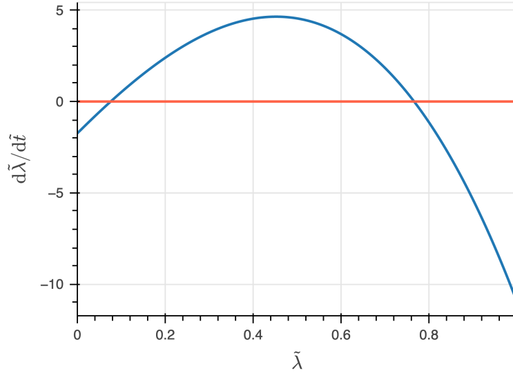
Figure 2: d\tilde{\lambda}/dt versus \tilde{\lambda} for parameters given in Table 2, assuming a growth rate of 0.7 \text{ hr}^{-1} , a_{\text{ex}} = 1 \text{ }\mu\text{M} , and q_{\text{ex},0}^{\text{max}} = 11.9 \text{ min}^{-1} .
