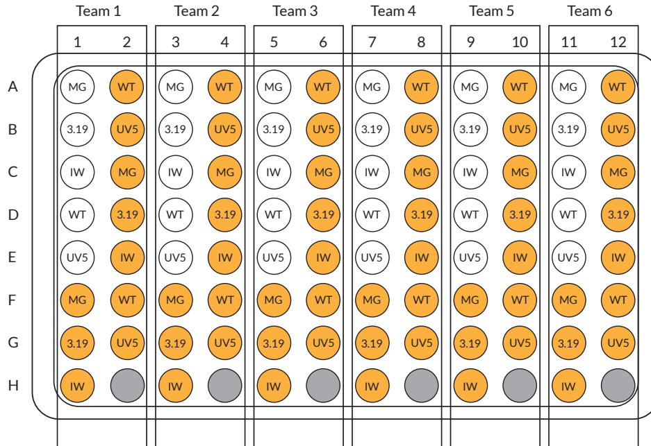
Figure 4: Plate layout for growth with antibiotic. White wells are media without antibiotic, i.e., M9 minimal media with 0.5% Glucose. Orange wells are for media with antibiotic. The gray well has media but no cells, left as a blank.
